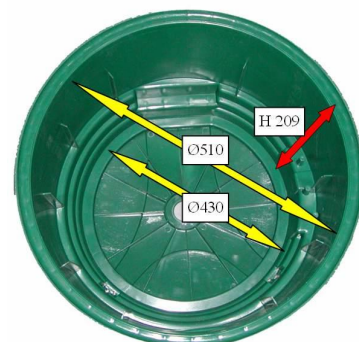
Round cap for vertical and spherical tanks
